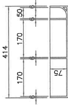
SECTION
